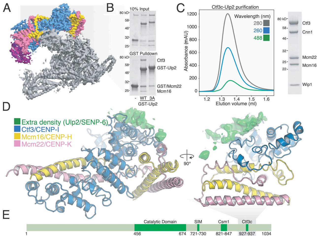
Figure 1. Reconstitution and structure of the Ctf3c-Ulp2 complex. (A) Model of the assembled Ctf19c (Ctf3, blue; Mcm22, pink; Mcm16, yellow; Cnn1/Wip1, purple; Chl4, Iml3, Ctf19, Mcm21, Ame1, Okp1, Nkp1, Nkp2, gray; and EMD-0523, EMD-21910; Hinshaw and Harrison, 2019; Hinshaw and Harrison, 2020). (B) The Ctf3c binds the Ulp2-KIM but not the Ulp2-KIM-3A peptide. Purified Ctf3c and GST-Ulp2-KIM were mixed and subjected to pull-down on glutathione beads. Input and pull-down samples were analyzed by SDS-PAGE. (C) Purification of the Ctf3c-Ulp2-KIM complex by size exclusion chromatography. Absorbance wavelengths are indicated (mAU, milli-absorbance units). 488 nm reports on the FITC-Ulp2-KIM peptide. Eluate from the peak fractions were analyzed by SDS-PAGE. (D) Structure of the Ctf3c-Ulp2 complex. Extra density corresponding to Ulp2-KIM is shown as a green surface derived from the final density map. (E) Domain diagram of Ulp2. Regions with known functions are annotated.
